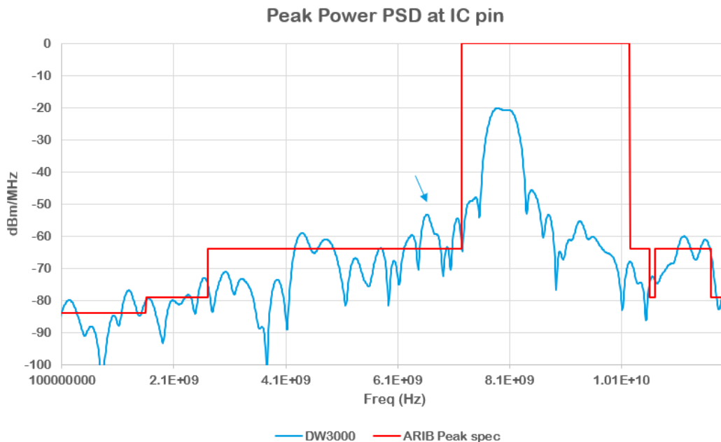
Figure 2 Typical DW3000 Peak Power when operating at maximum power level
