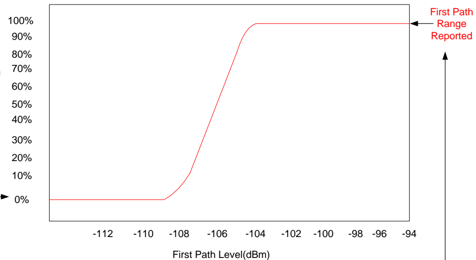
Fig: C. DW1000 performance for NLOS with single reflection
