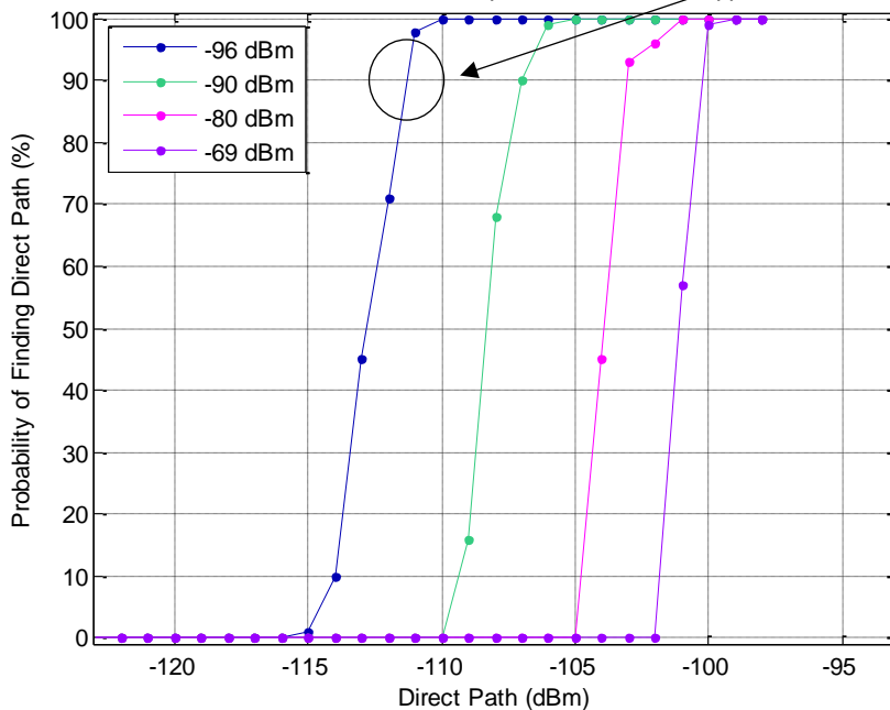
Figure 9: Multipath with preamble length of 1024
