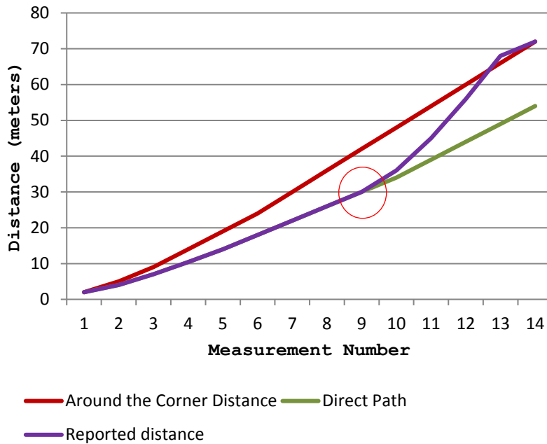
Figure 20: Extrapolation of the test results when applying new threshold settings
