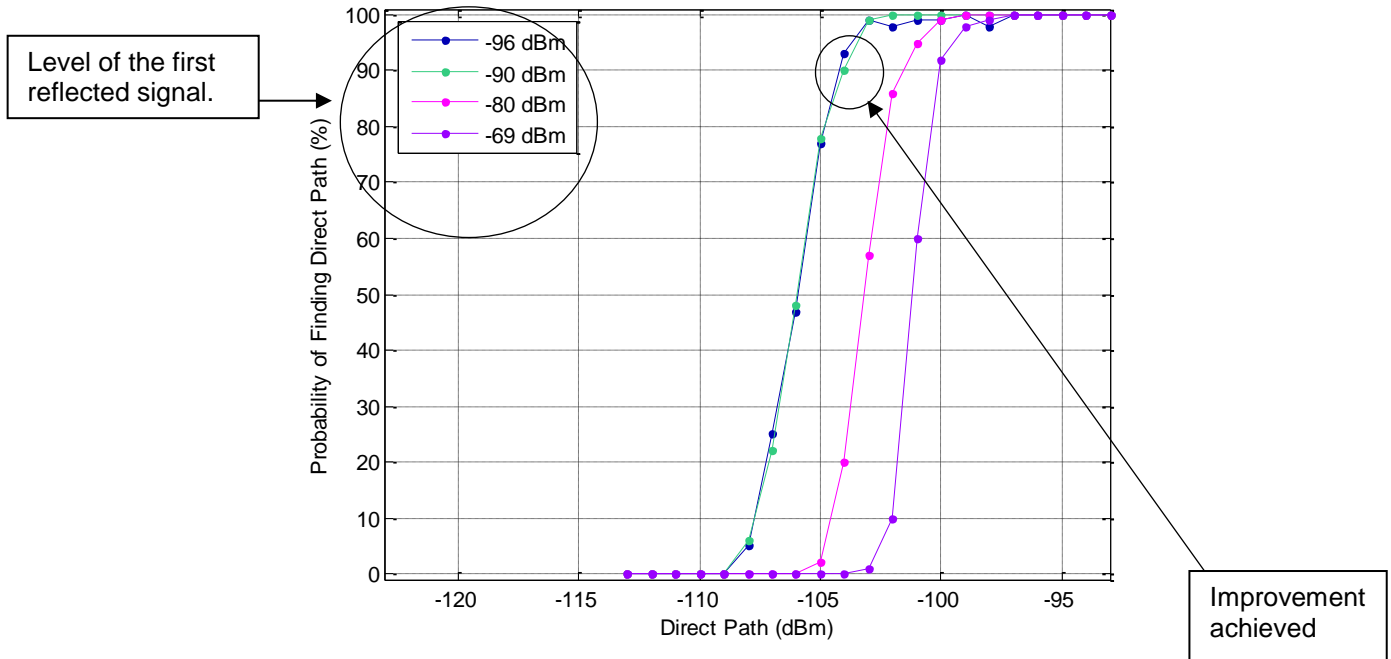
Figure 8: Multipath with preamble length of 128
