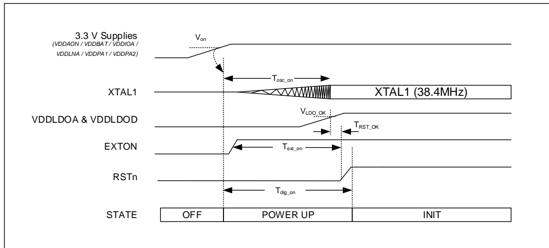
Figure 2: DW1000 power up sequence
