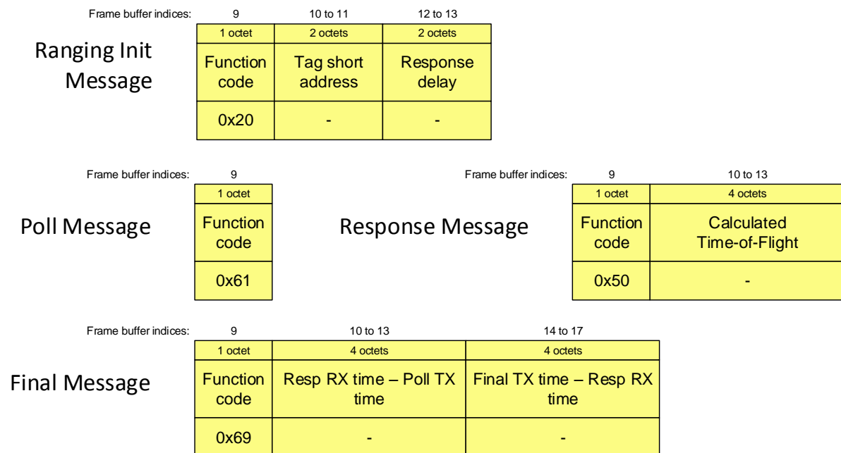
Figure 5: Ranging message encodings
