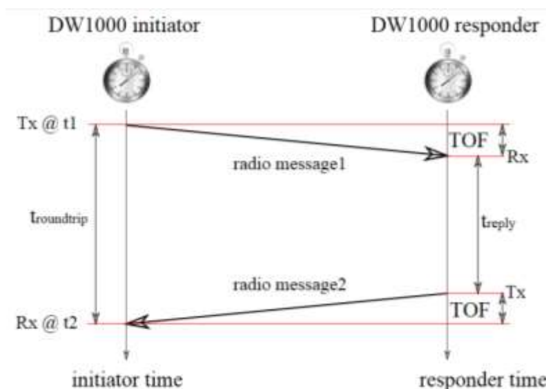
Figure 1: Two-way ranging concept
