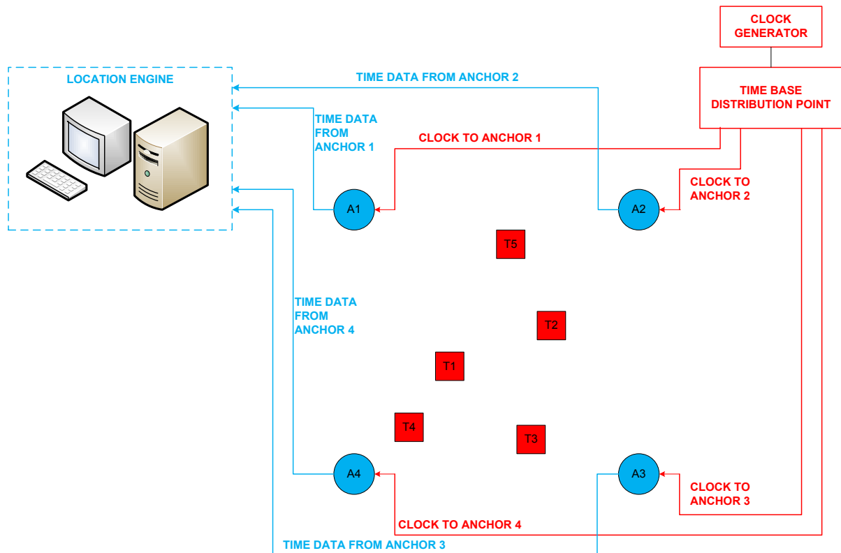
Figure 1: Basic concept of a wired synchronization scheme
