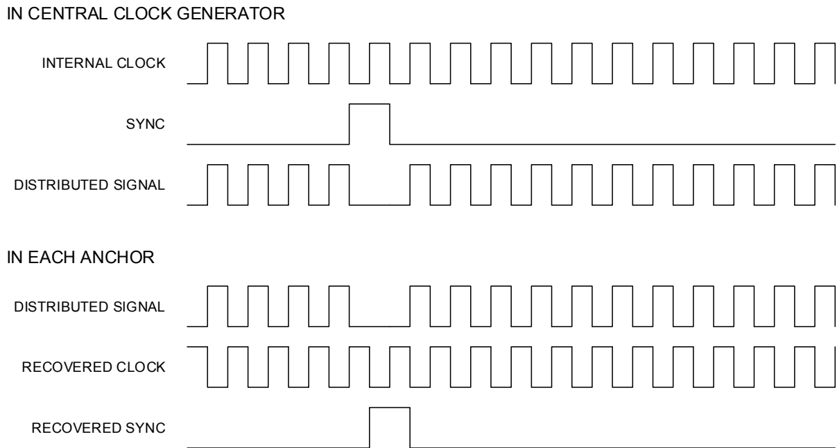
Figure 6: Using a clock violation to distribute the SYNC signal
