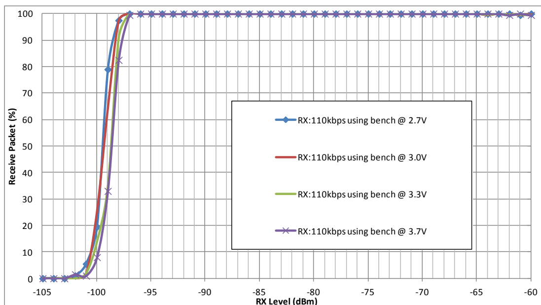
Figure 7: RX Sensitivity versus supply voltage for 110 kbps data rate
